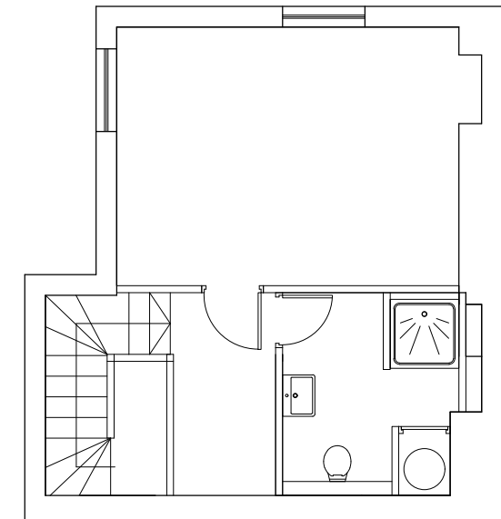
Fifth Floor
